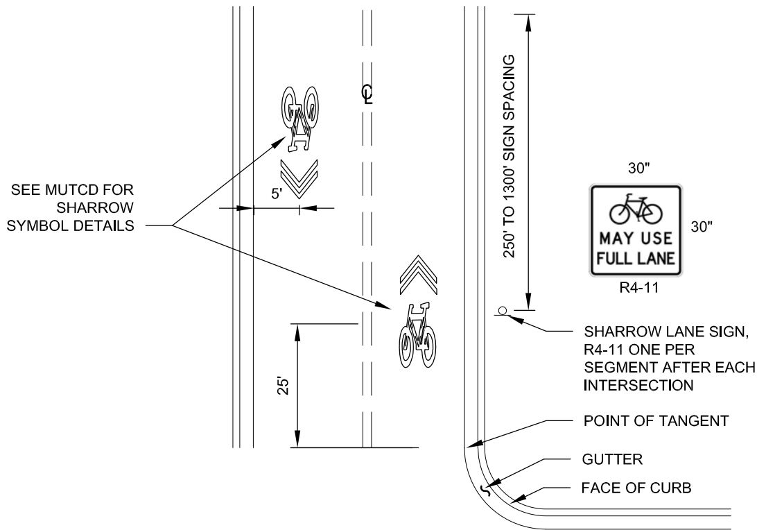
TYPICAL SHARROW LAYOUT NTS
