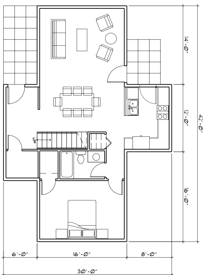
HOUSE B PLAN 2
