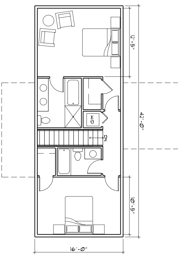
HOUSE B UPPER LEVEL PLAN 1
